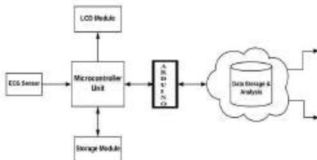
Fig.2.Sending End
